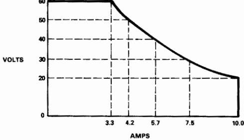
Autoranging operating area for the 6024A
