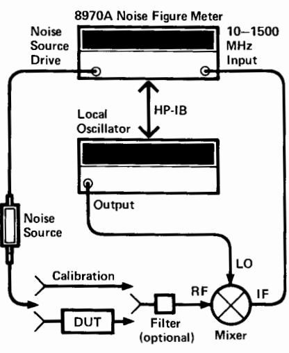
Figure 4. Swept microwave amplifier measurement.
