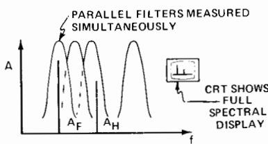
Figure 1c. Fourier analyzer
