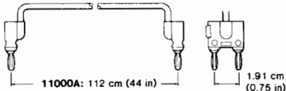
11000A: 112 cm (44 in) 1.91 cm (0.75 in)
