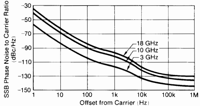
Typical System Sensitivity (when used with the 8662A)
