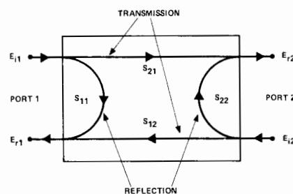
Figure 7. S-parameter model for a two-port linear network
