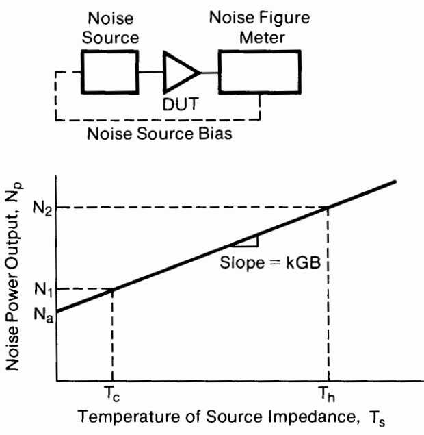
Figure 3. Available noise power and noise figure measurement.
